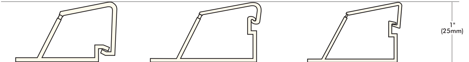
1" EASED EDGE SIDE LOAD
