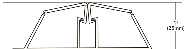
1" MICRO EASED EDGE MIDWALL (IN DEVELOPMENT)
