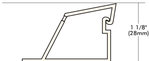
1 1/8" SQUARE TOP LOAD
